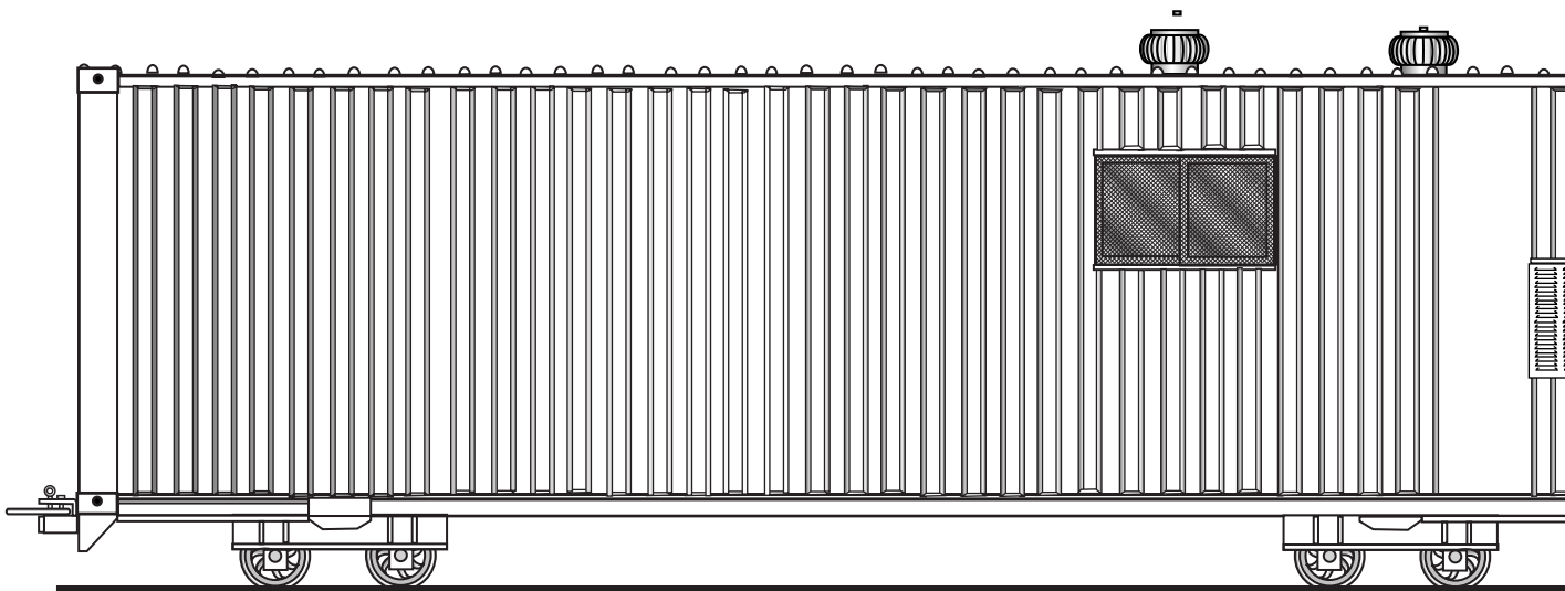
Side Elevation
